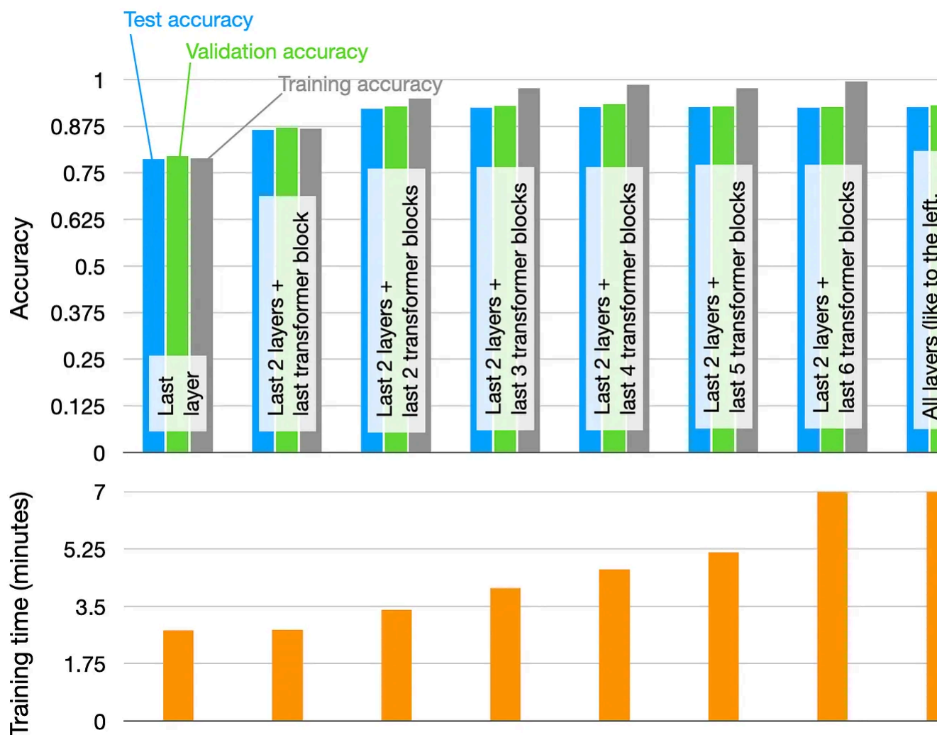
Performance of pretrained DistilBERT models finetuned on the IMDB Movie review dataset. The code can be found here on GitHub .
